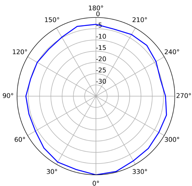
2.4GHz (Horizontal)
